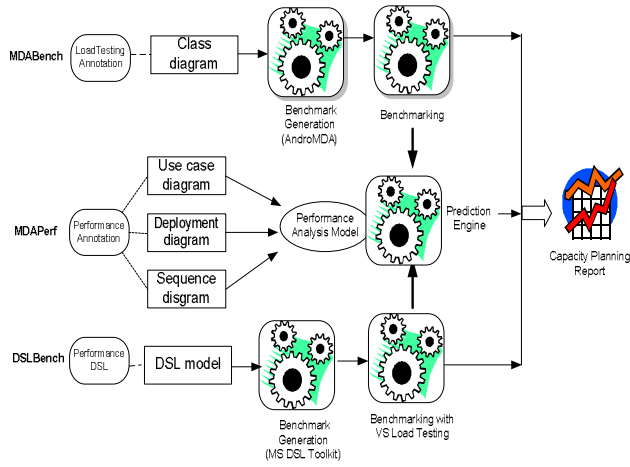
Figure 1. Revel8or Model Driven Capacity Planning Toolkit
