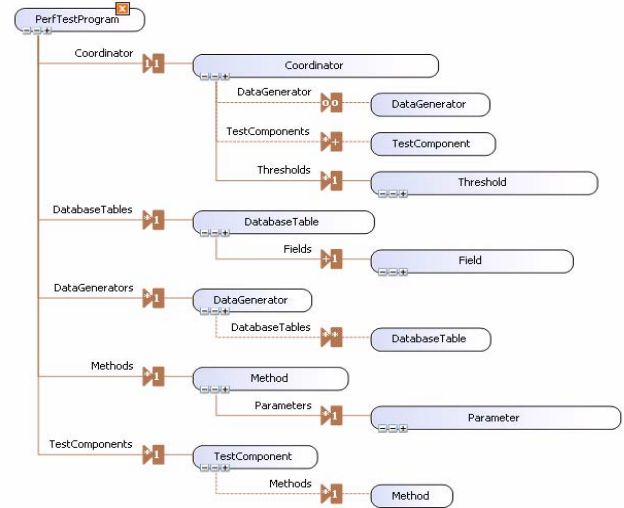
Figure 3: Meta-model for performance testing domain
